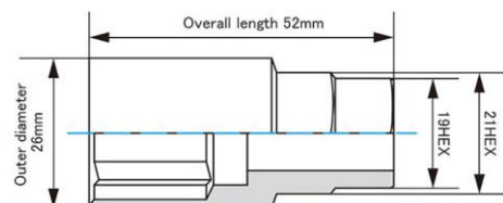
■KEY ADPTER (A93K)
